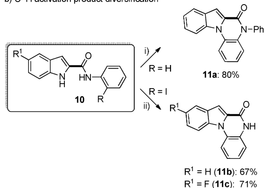
Scheme 7. Diversification of C–H activation products. Reagents and conditions: i) 1-Fluoro-2-nitrobenzene, Cs 2 CO 3 , CH 3 CN, 90 °C, 12 h. ii) CuI (cat.), L-proline (cat.), NaH, DMF, 150 °C, μw, 5 min.
